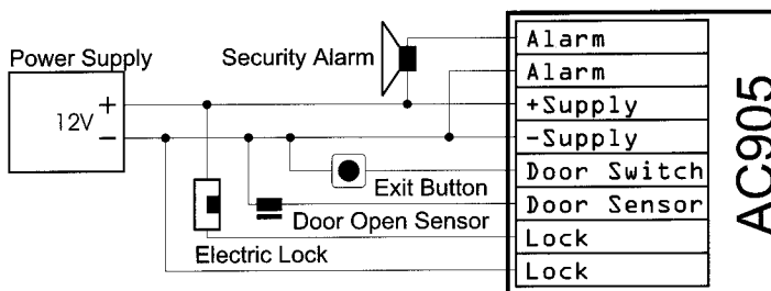
Typical AC905 Wiring Diagram
